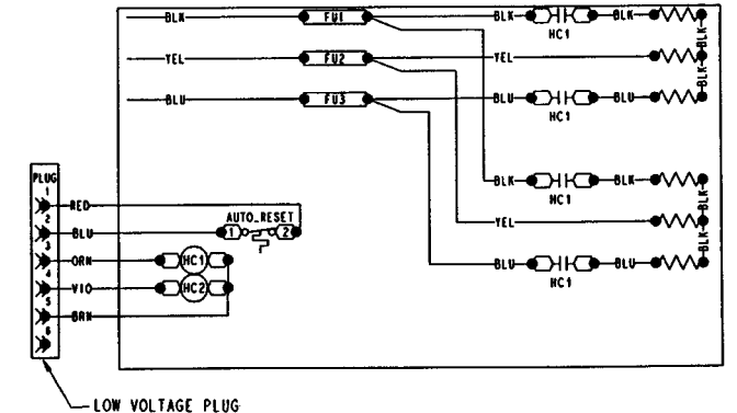
CRHEATER129A00, 135A00 (600 V, 36 kW†)
